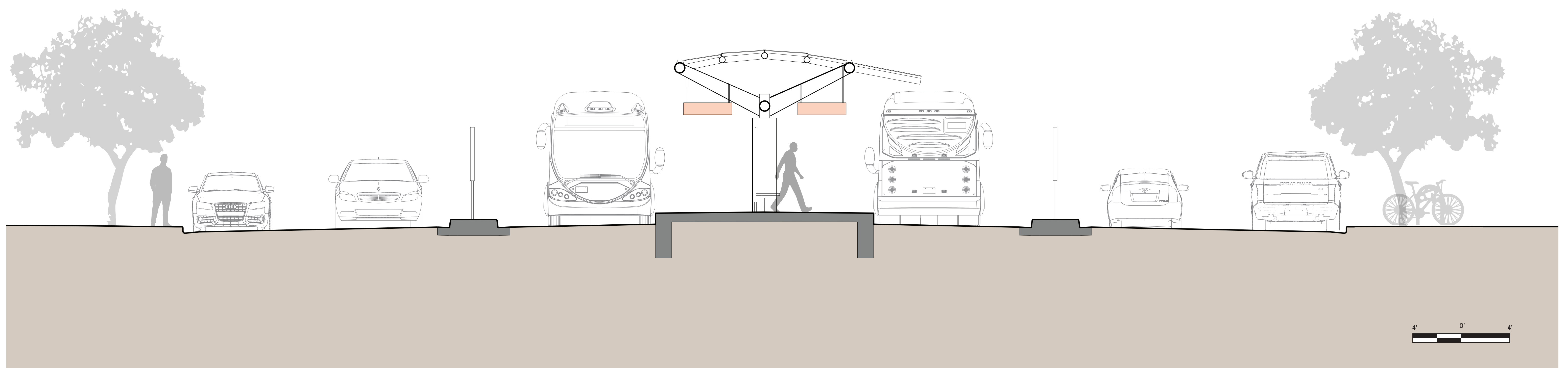
Section
