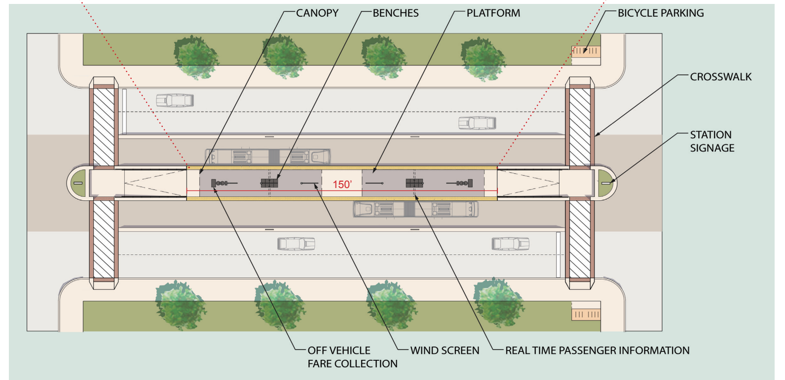
STATION PROTOTYPE
