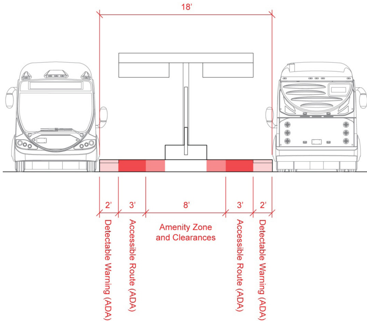
SIZING DIAGRAMS
